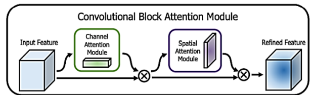
Figure 3. Spatial and channel attention modules can be applied sequentially or in parallel (Woo et al., 2018).
