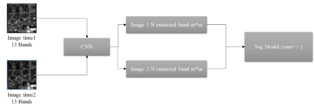
Figure 3. Feature extraction model architecture.
