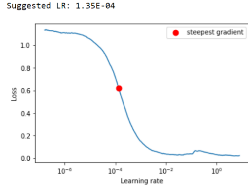
Figure 2. Learning rate finder curve. The x-axis is the learning rate (log scale), and the y-axis is the training loss (MSE). The optimal rate (marked by the red dot at \sim 1.35e-4 ) corresponds to the steepest negative slope, indicating fastest convergence before divergence.
